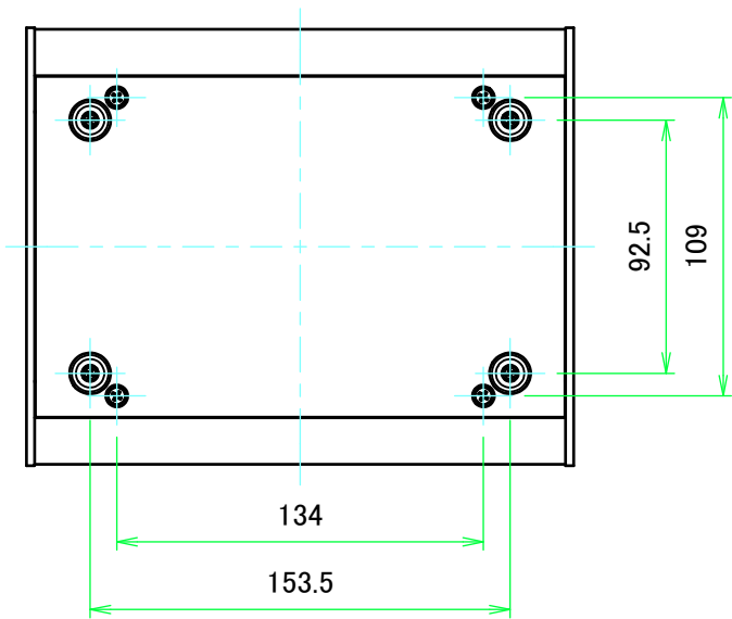
F view
