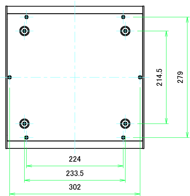
F view
