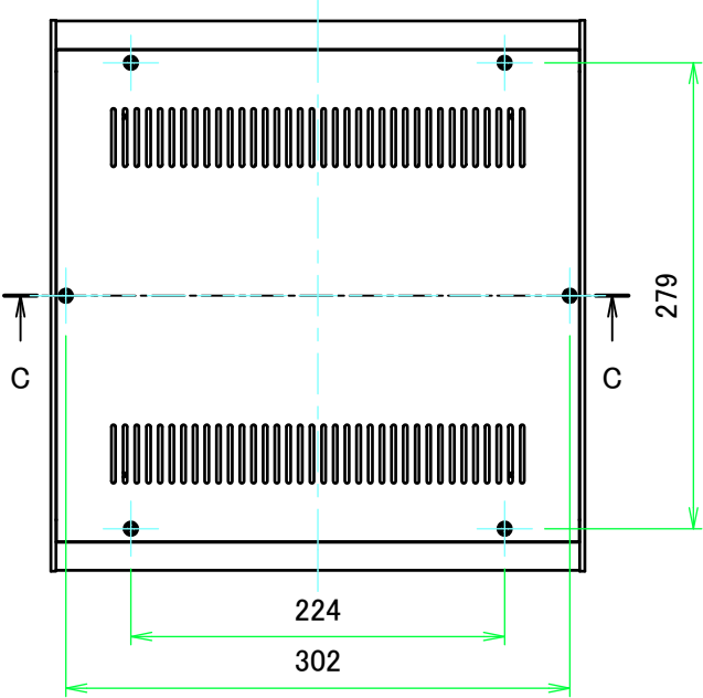
A view
