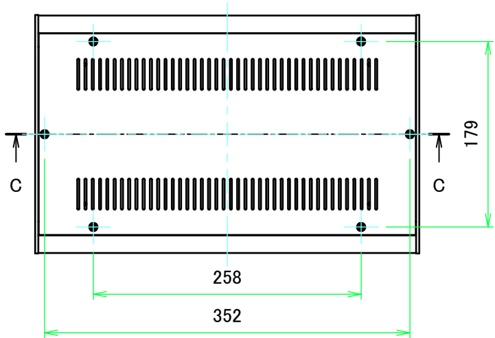
E view
