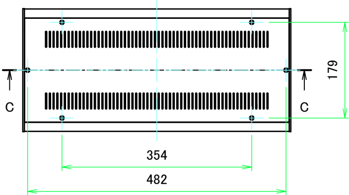
E view
