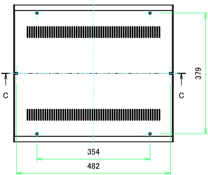
E view
