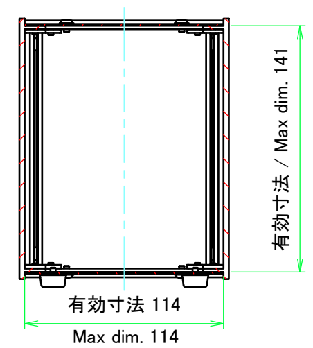
C-C (1:3)
