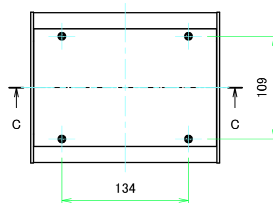
E view
