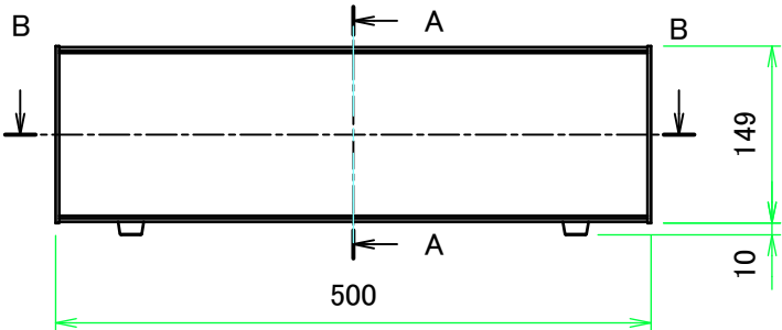
A view
