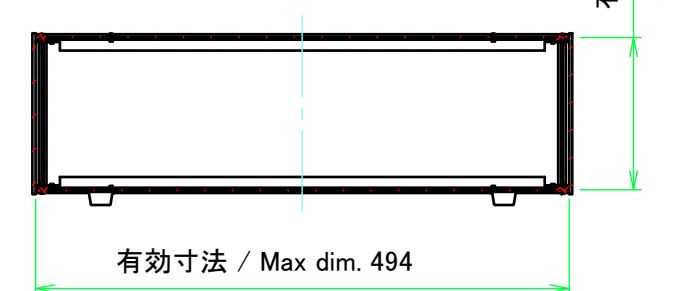
C-C (1:7)
