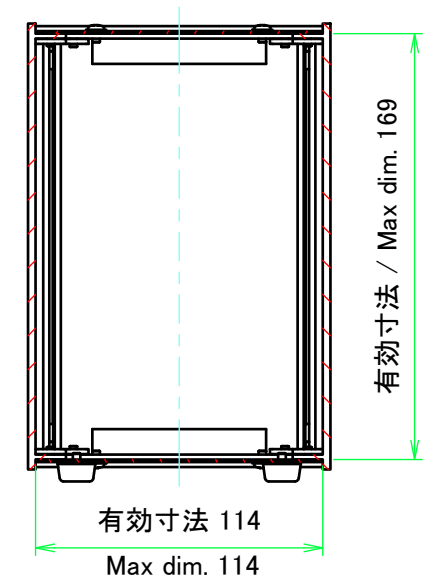
C-C (1:3)
