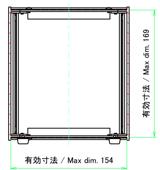
C-C (1:3)
