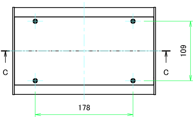
E view
