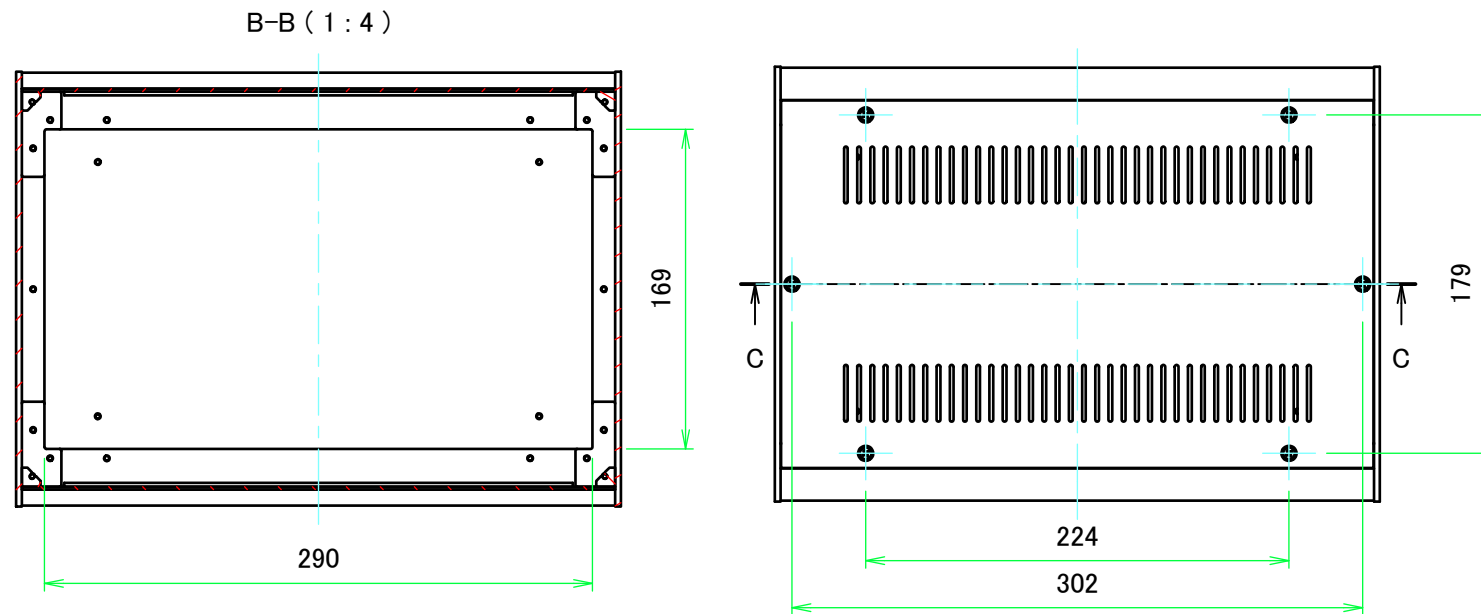
E view
