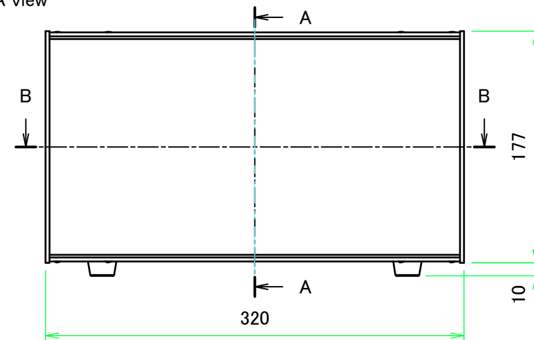
A view
