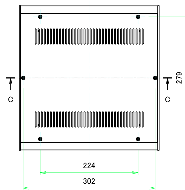
E view
