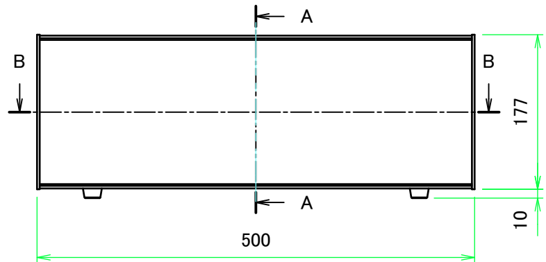
F view
