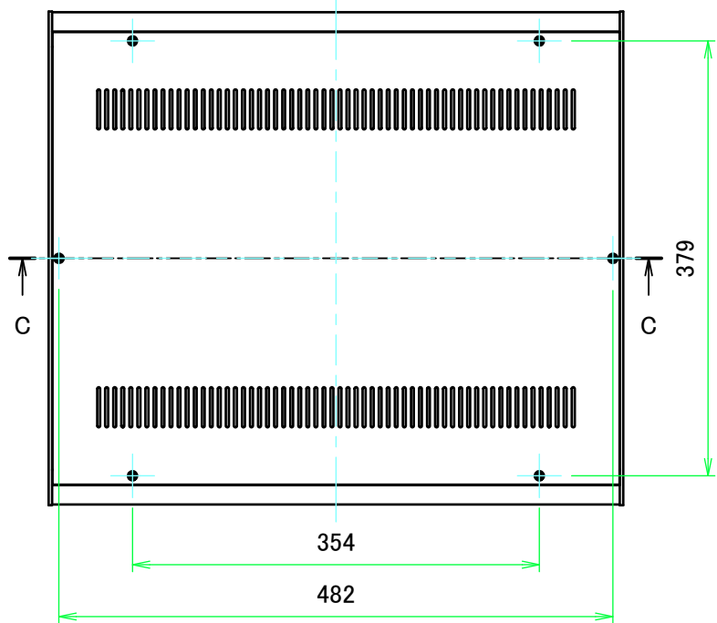
A view
