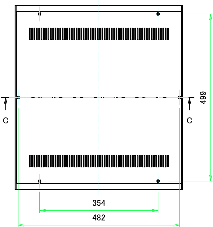
A view
