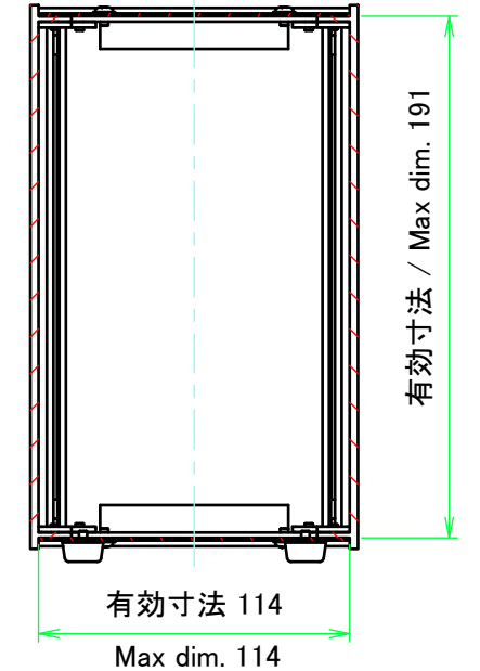
C-C (1:3)
