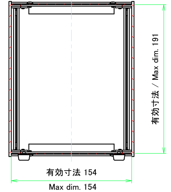
B view
