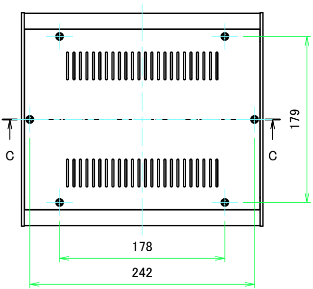
A view
