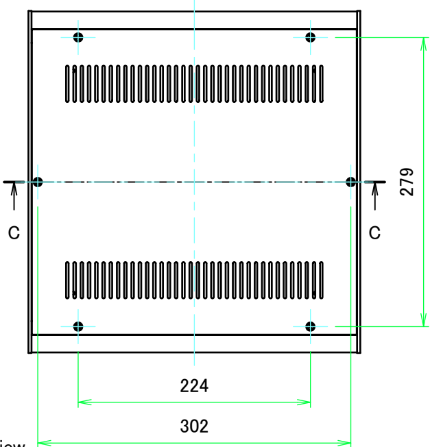
A view
