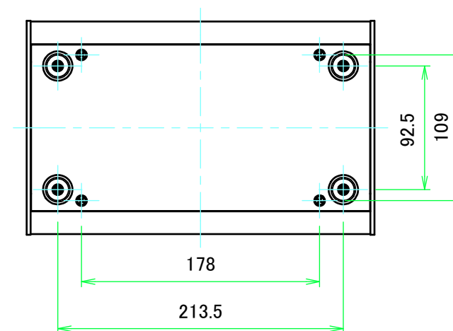
F view
