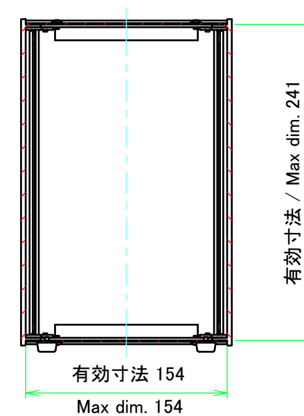
B view
