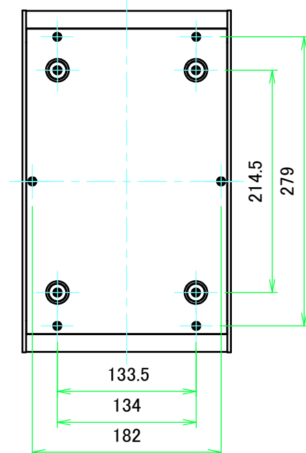
F view
