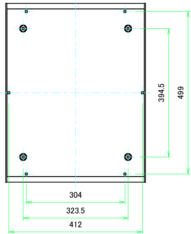
F view
