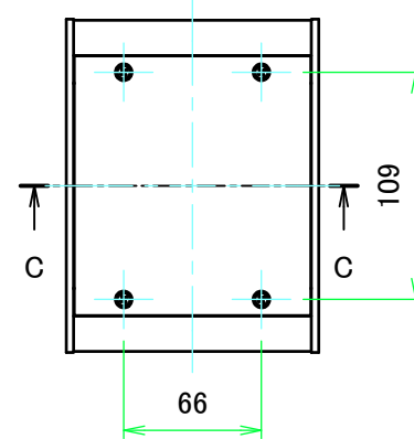
E view
