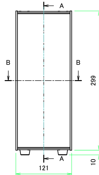
F view
