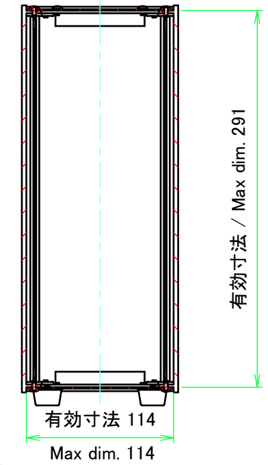
B view
