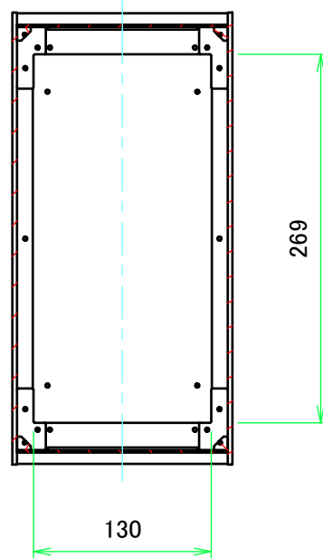
B-B (1:5)
