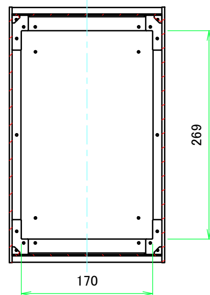
B-B (1:5)
