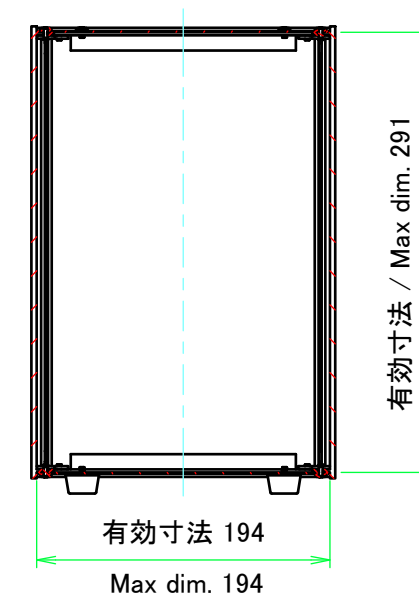
C-C (1:5)
