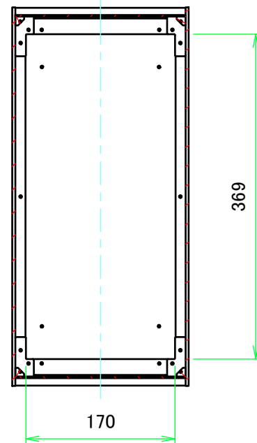
B-B (1:6)
