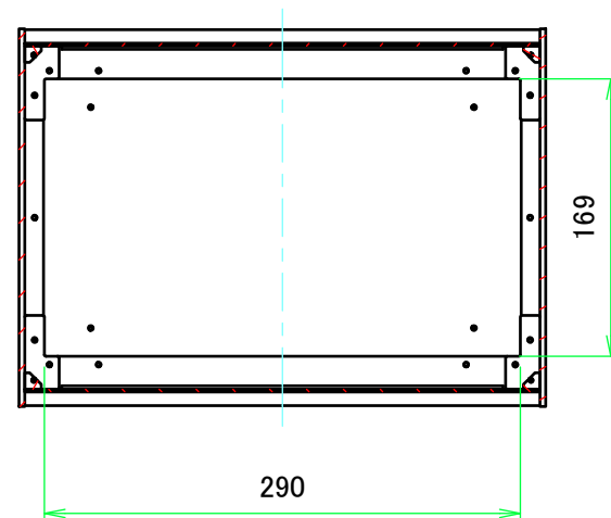
B-B (1:5)
