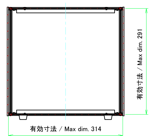
C-C (1:5)
