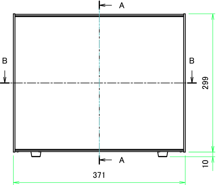
A view
