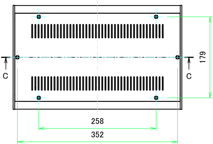
E view
