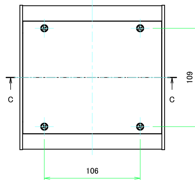
A view
