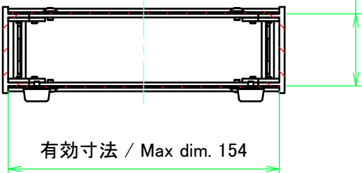
C-C (1:3)
