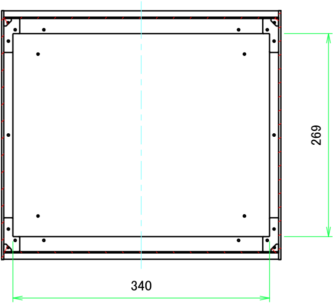
D view
