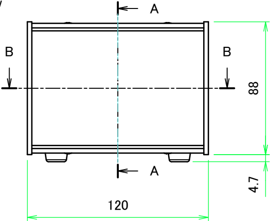
A view
