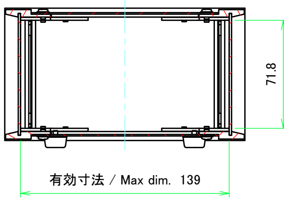
C view
