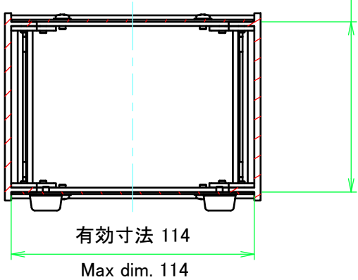
B view
