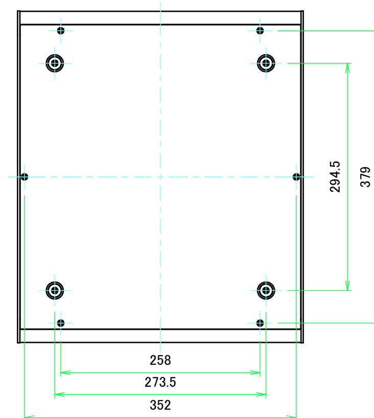
F view
