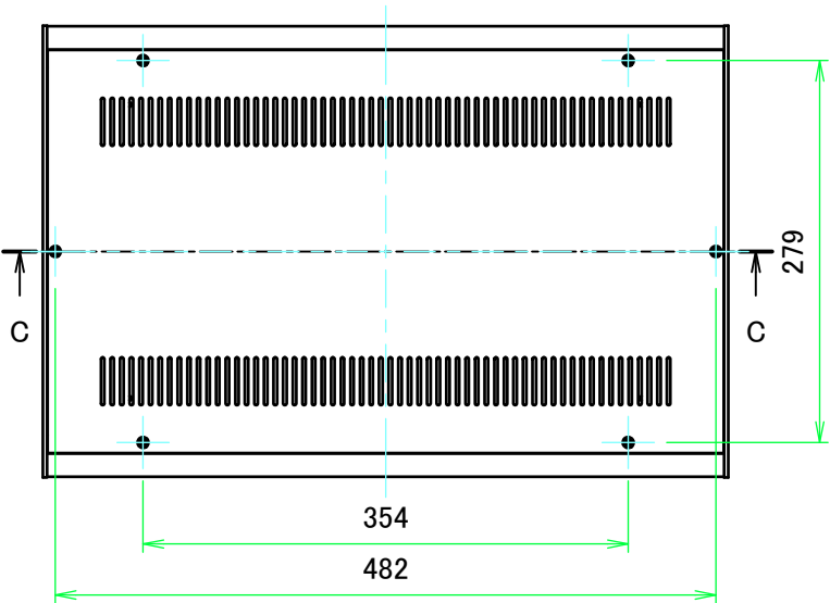
A view
