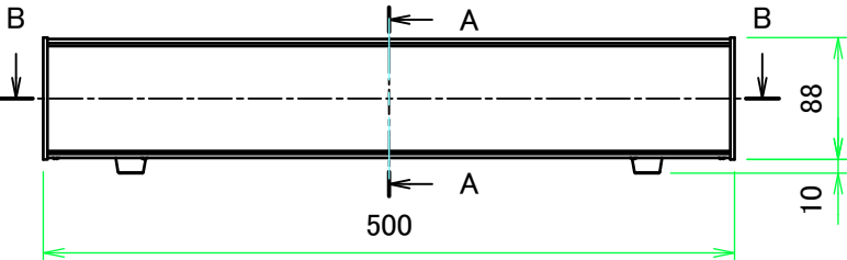
A view
