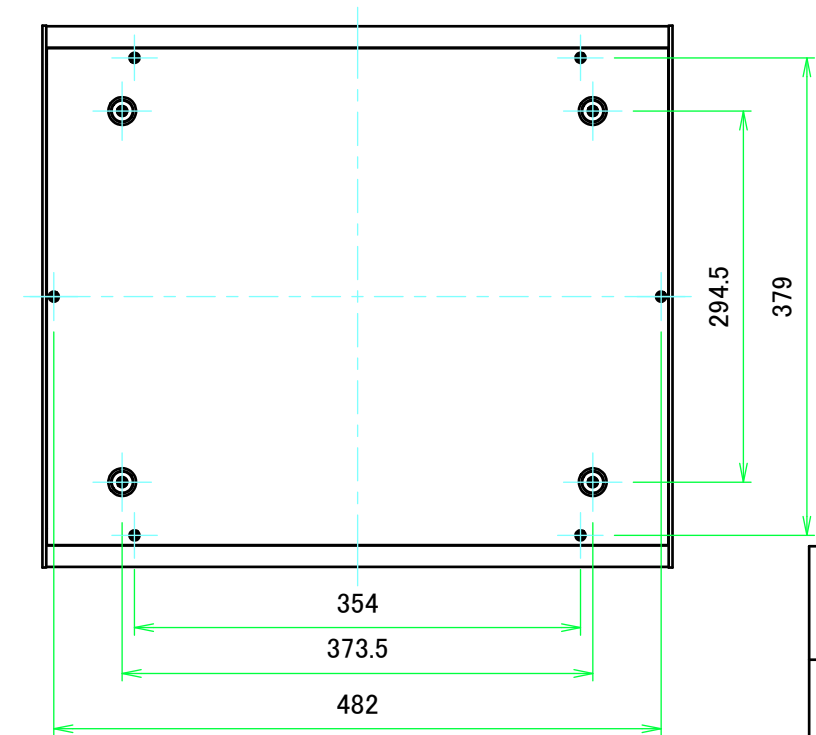
F view
