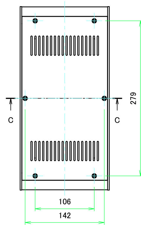
A view
