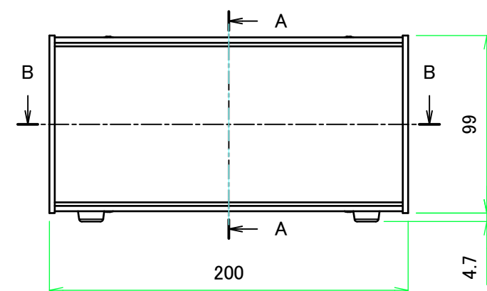
F view
