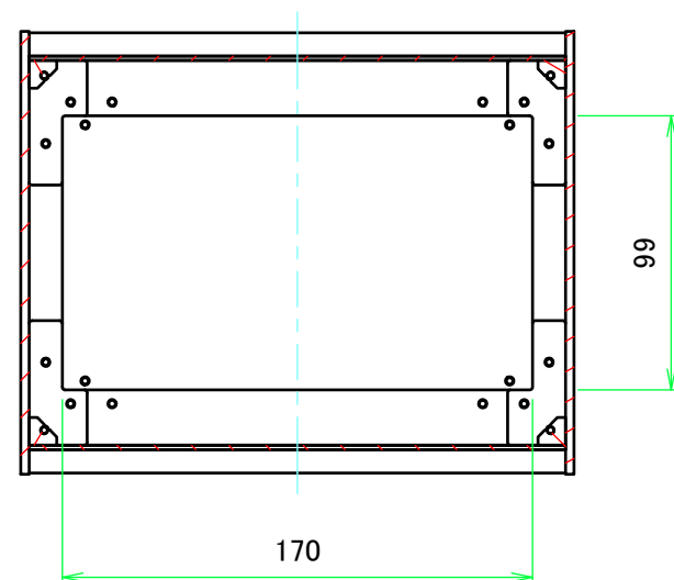
B-B (1:3)
