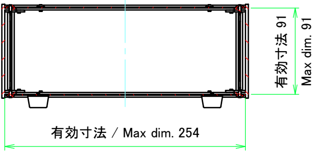
C-C (1:4)
