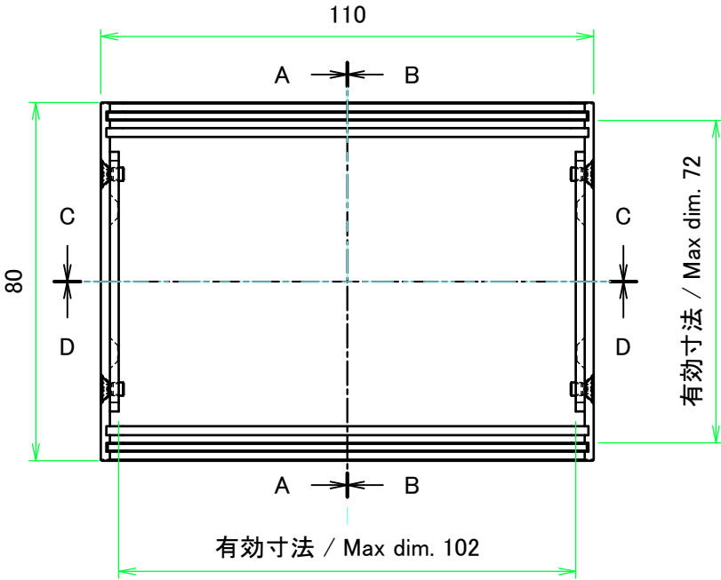
下カバー(内視) Bottom cover (Internal view)
