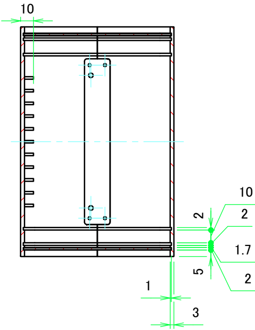
B-B (1:3)
