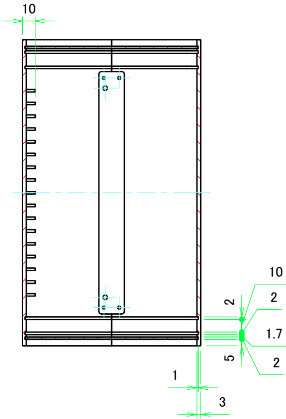
B-B (1:3)
