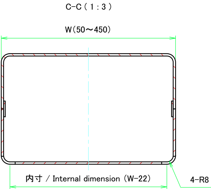
下カバー(内視) Bottom cover (Internal view)
