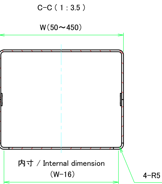
下カバー(内視) Bottom cover (Internal view)
