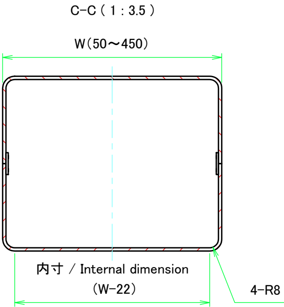
下カバー(内視) Bottom cover (Internal view)
