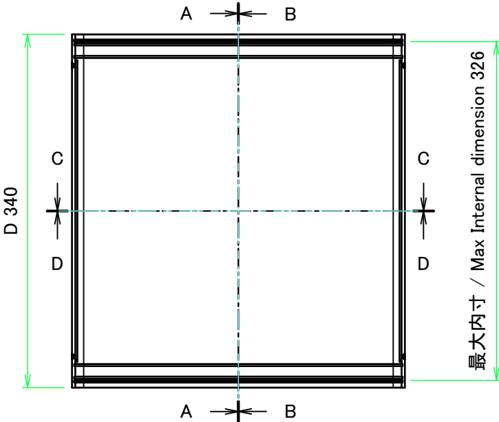
下カバー(内視) Bottom cover (Internal view)
