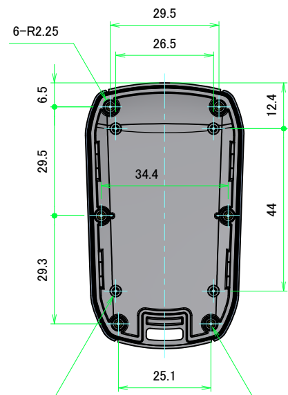
C-C (1:1)
