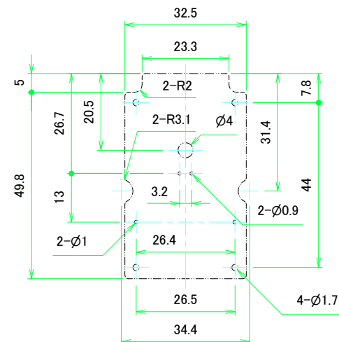
推奨基板形状 / Recommended PCB dimension
