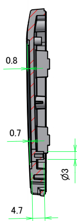
C-C (1:1)
