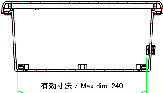
B-B (1:4)
