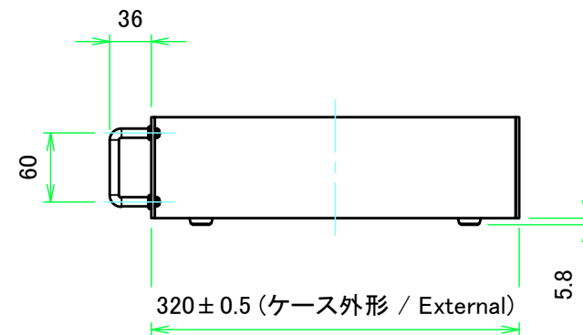
C view
