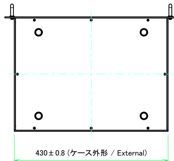
F view
