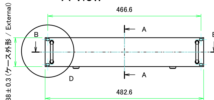
A view
